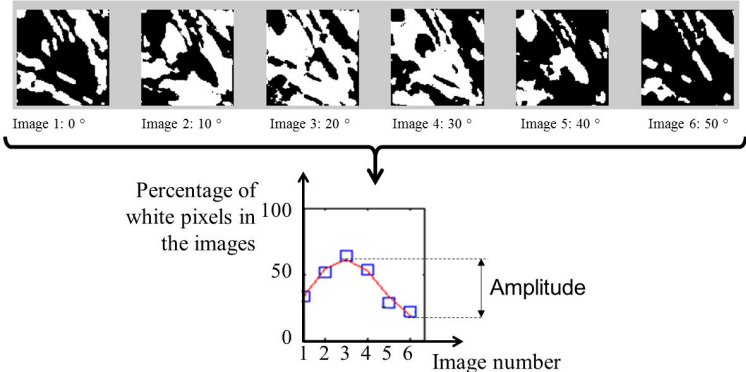
Figure 10: View of binary images from Figure 9 and evolution curve of the white pixels percentage according to the six consecutive images.
