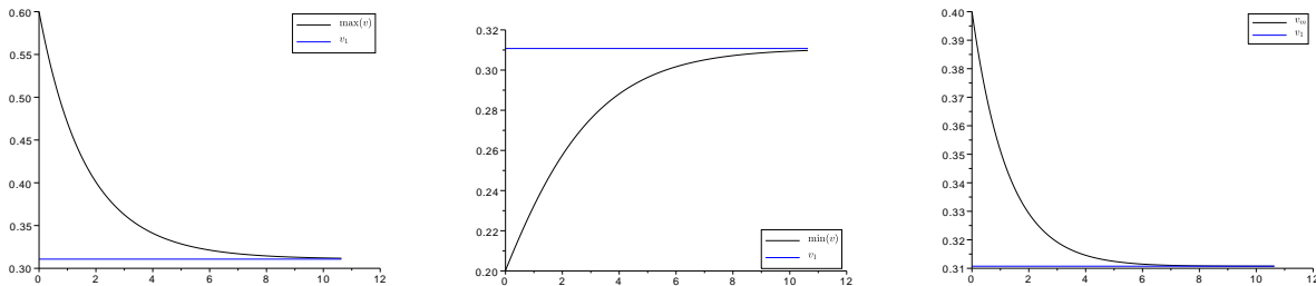
Figure 3: Convergence in time (black line) of the maximum (left), the minimum (middle) of v(t, \cdot) , and of mean value v_m(t) (right) towards the value v_1 = 0.3107435 (blue line) for the parameters \rho = 0.7 , a = 0.25 , b = 0.5 , \varepsilon = 0.35 and \sigma = 1 .
