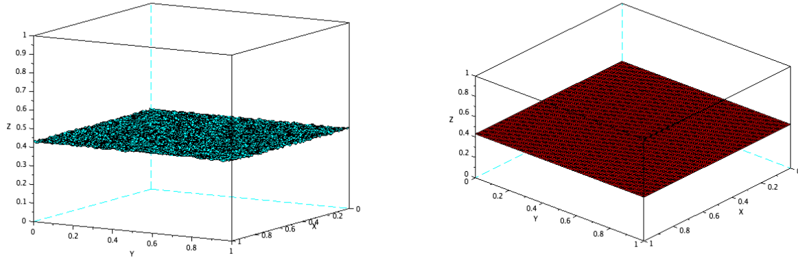
Figure 1: The initial data (left) and the equilibrium solution (right) for the function v . The parameters used for the computation are : \rho = 1 , a = 0.25 , b = 0.5 and \varepsilon = 0.35 , \sigma = 1 and T = 200 .
