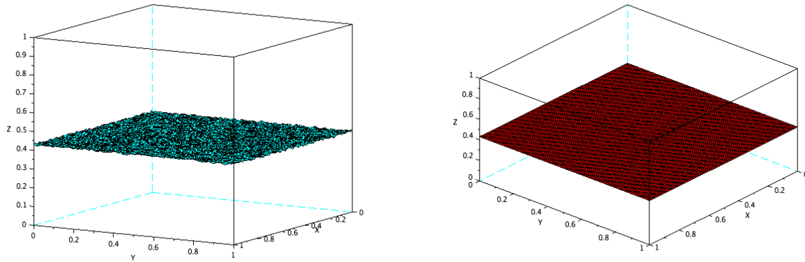
Figure 1: The initial data (left) and the equilibrium solution (right) for the function v . The parameters used for the computation are : \rho = 1 , a = 0.25 , b = 0.5 and \varepsilon = 0.35 , \sigma = 1 and T = 200 .
