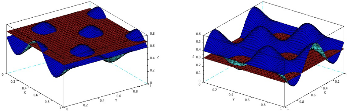
Figure 2: The initial data (blue) and the equilibrium solution (red) for the functions u (left) and v (right). The parameters used for the computation are : \rho = 0.7 , a = 0.25 , b = 0.5 and \varepsilon = 0.35 , \sigma = 1 and T = 10 .
