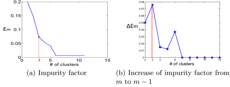
Fig. 4. Determination of cluster number by impurity factor
