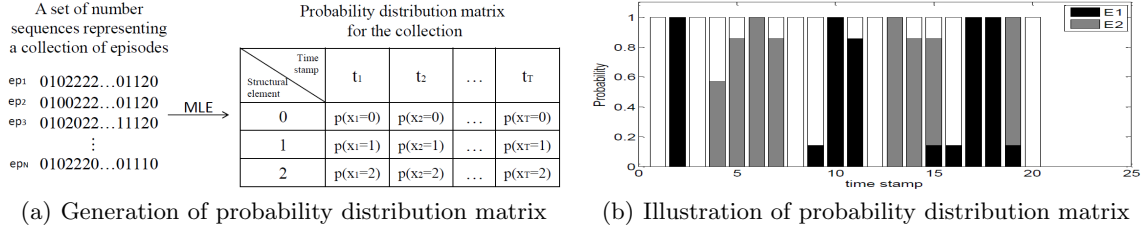
Fig. 3. Structure modeling for unique structure with two structural elements.
