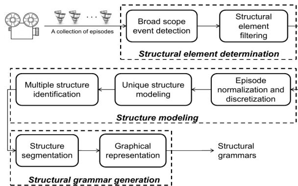
Fig. 1. General architecture of the three-stage approach for the grammatical inference of program structuring.
