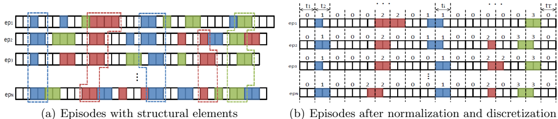
Fig. 2. An example of structural element determination and episode pre-processing
