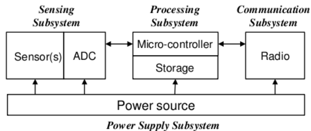
Fig. 1: Functional subsystems of a wireless sensor node
