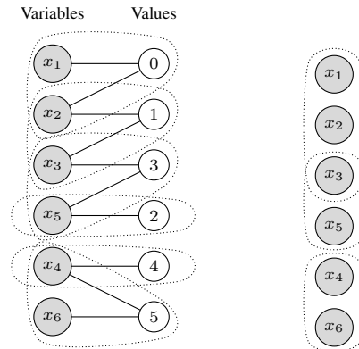
(a) f^{val} = \{\{x_1, x_2\}, \{x_2, x_3\}, \{x_3, x_5\}, \{x_4, x_6\}\} . (b) A possible multifunction f_{\mathcal{P}}^{val}(\mathcal{X}) = \{\{x_1, x_2, x_3\}, \{x_3, x_5\}, \{x_4, x_6\}\} .
