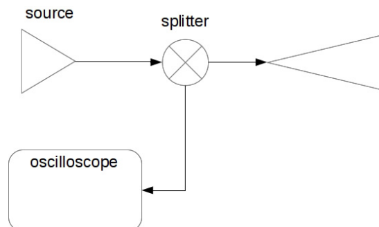
Figure 10. Experiment set-up.
