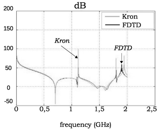
Figure 9. Comparison with a Finite Difference Time Domain computer code.
