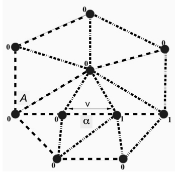
Figure 1. Spanning tree.
