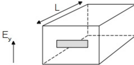
Figure 7. Electric field on cavity with an aperture.
