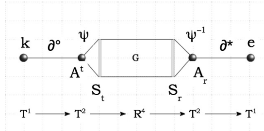
Figure 6. Sequence of operation for free field.
