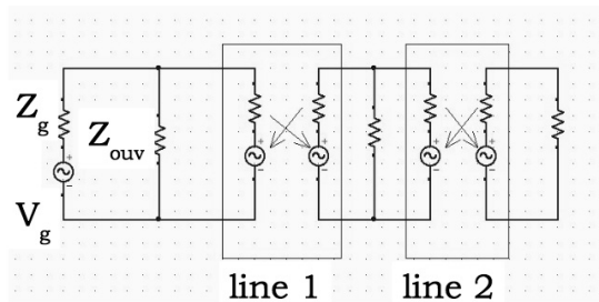
Figure 8. Kron's model for a cavity.
