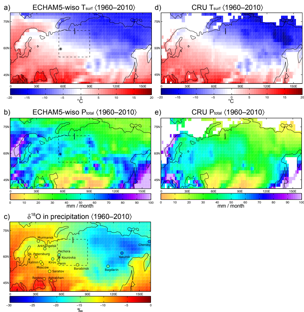
Figure 1. Left column: simulated mean annual values of (a) surface temperature, (b) precipitation, and (c) \delta^{18}\text{O} in precipitation, averaged over the period 1960–2010. Right column: CRU data of (d) surface temperature, and (e) precipitation amount, averaged over the same period. The circles in Fig. 1c mark the position of the various GNIP stations used for analyses in this study.
