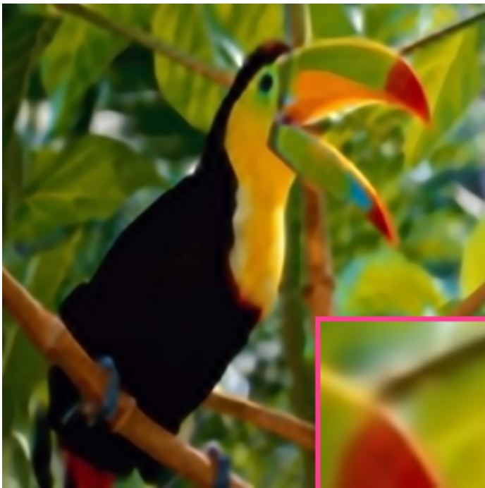
Algorithm 2
