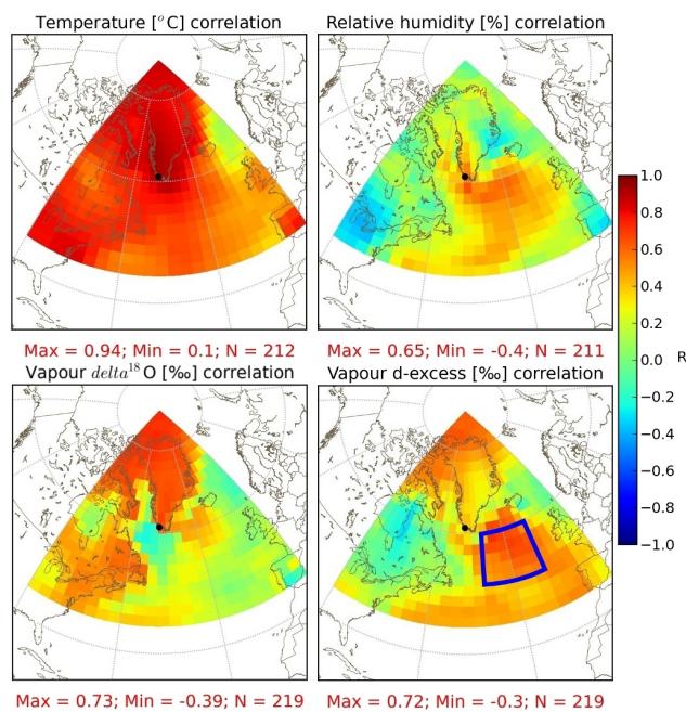
Fig. 12. Maps of correlations between Ivittuut daily observations and LMDZiso simulated daily values at different grid cells, for temperature, relative humidity, \delta^{18}\text{O}_{\text{v}} and d_{\text{v}} . Colour indicates R correlation coefficient. Blue square on lower right box represents the region called “Zone 1”.
