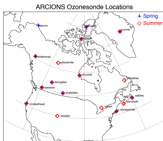
Figure 8. Location of ARCIIONS ozonesonde sites used in April and June–July 2008 in coordination with ARCTAS.
