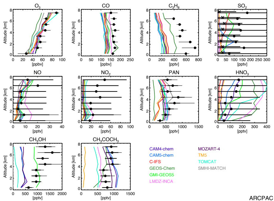
Figure 17. As Fig. 16, for ARCPAC NOAA P3 observations.
