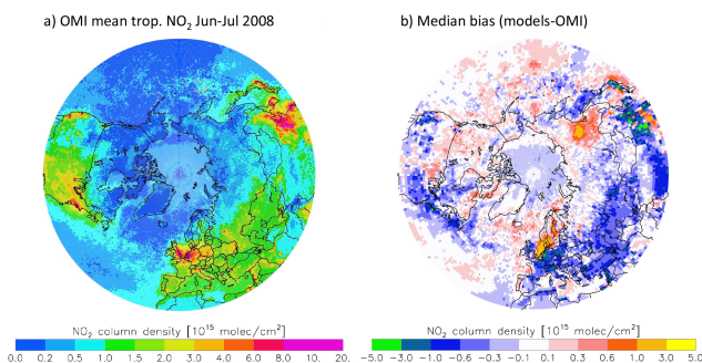
Figure 12. (a) OMI tropospheric column \text{NO}_2 and (b) median of the model biases, both for 18 June–15 July.
