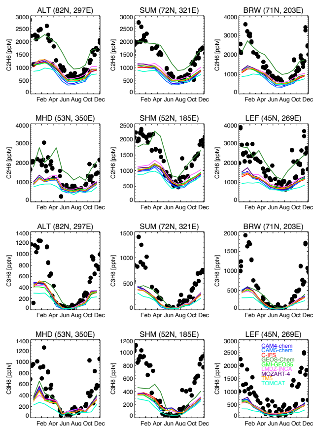
Figure 11. Ethane (top six panels) and propane (lower six panels) at several Northern Hemisphere NOAA GMD network sites. Monthly mean model output (colored lines) is plotted with 2008 weekly observations (black circles). Station codes: ALT: Alert, Canada; SUM: Summit, Greenland; BRW: Barrow, Alaska; MHD: Mace Head, Ireland; SHM: Shemya, Alaska; LEF: Wisconsin.
