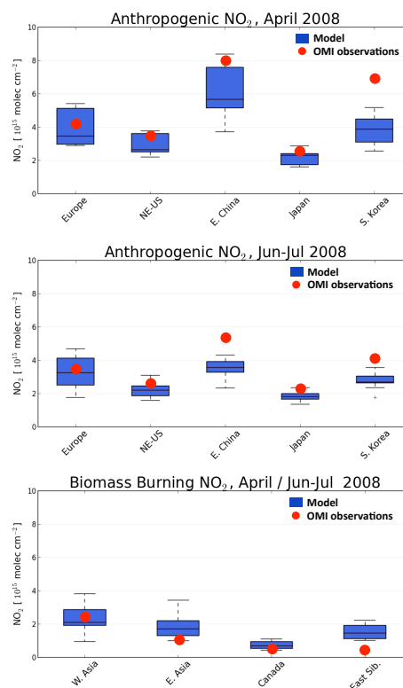
Figure 14. Summary of the regional means from each model and the OMI \text{NO}_2 tropospheric columns for each region indicated in Fig. 13. (top) Anthropogenic emissions in April and (middle) June–July, (bottom) biomass burning in both seasons. Red circles are mean OMI \text{NO}_2 observations for the region; box plots show median, 25th and 75th quartiles, whiskers to 5th and 95th percentiles of the model means.
