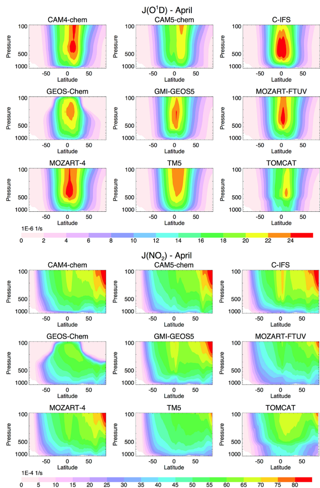
Figure 4. Zonal averages of photolysis rates for each model for April of J(O_3 \rightarrow O^1D) (top) and J(NO_2) (bottom).
