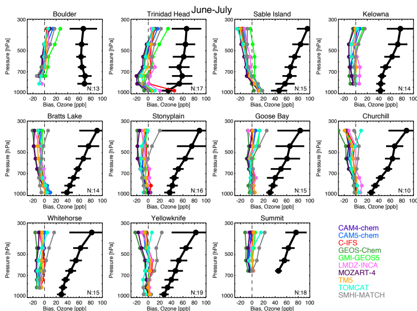
Figure 10. As Fig. 9, but for June–July.
