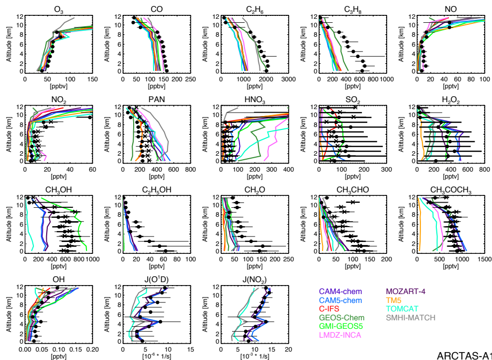
Figure 16. Comparison of model results interpolated to flight tracks of observations during the first four DC-8 flights of ARCTAS-A. Each profile is the median of 1 km altitude bins. Medians of observations in each 1 km altitude bin are shown as black circles and crosses (if a second measurement exists for a given parameter). Thick error bars represent the measurement uncertainty; thin error bars span inter-quartile range of all observations.
