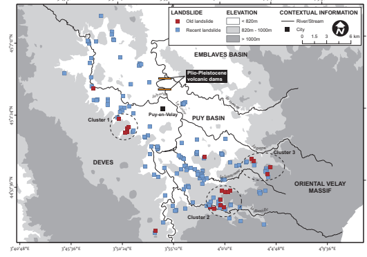
Figure 3 – Location map of inventoried landslide
