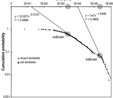
Figure 6 – Frequency-magnitude distribution of landslides of Puy-en-Velay basin
