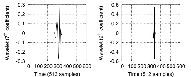
Figure 2. Daubechies-wavelet time variation for 2 different scaling factors
