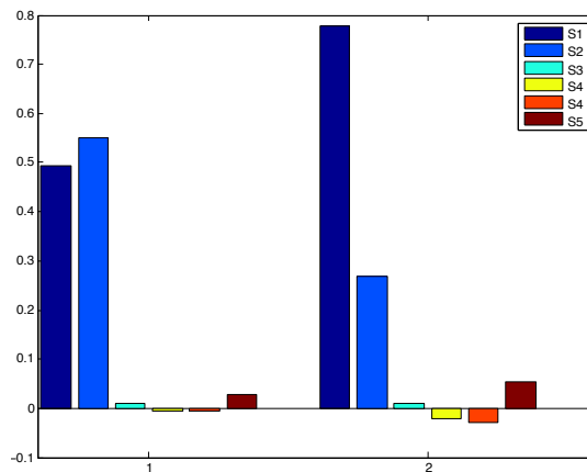
Figure 3: Sensitivity indices for the 6 inputs, at the ground floor (1) and at the first floor (2)
