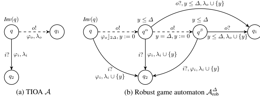
Fig. 3: Construction of the robust game automaton \mathcal{A}_{\text{rob}}^{\Delta} from an original automaton \mathcal{A} .
