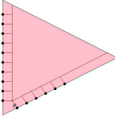
Figure 2: K -multiplicities and ancestors
