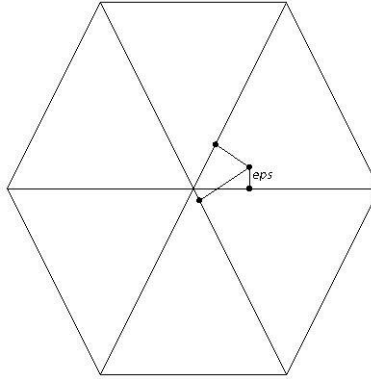
Figure 10: The point \epsilon and its projections \epsilon_\Delta
