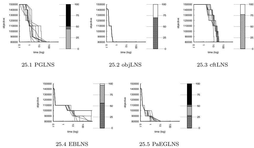
Fig. 25 league_model50-4-4.
