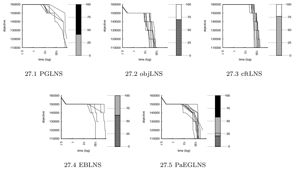
Fig. 27 league_model190-18-20.
