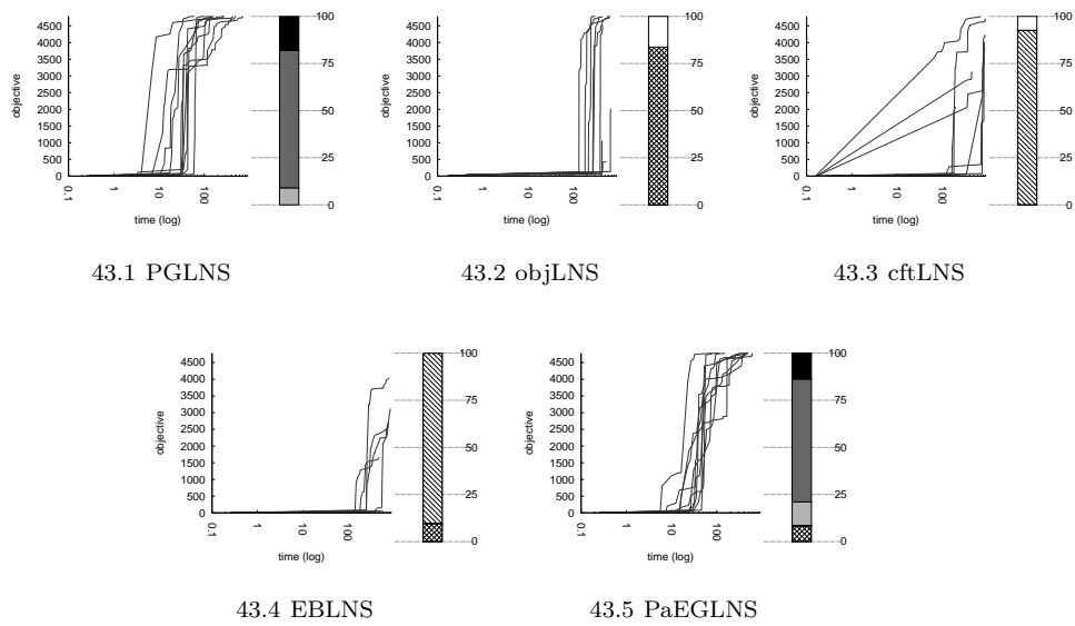
Fig. 43 pattern_set_mining_k1_ionosphere.
