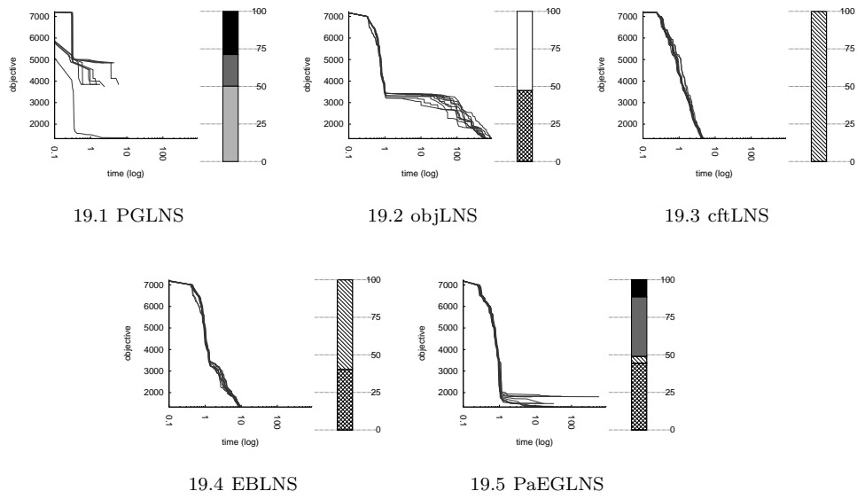
Fig. 19 fastfood_ff58.
