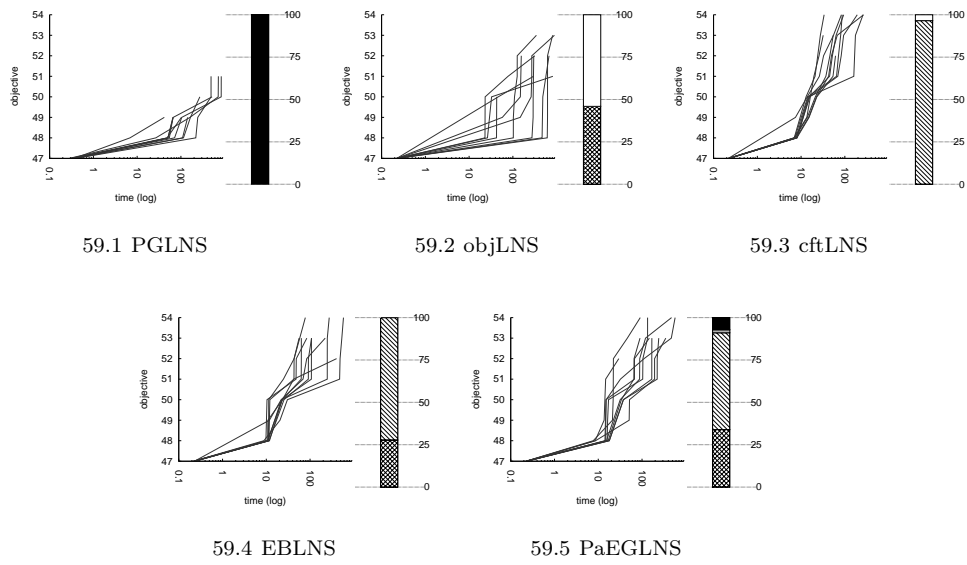
Fig. 59 still-life_11.
