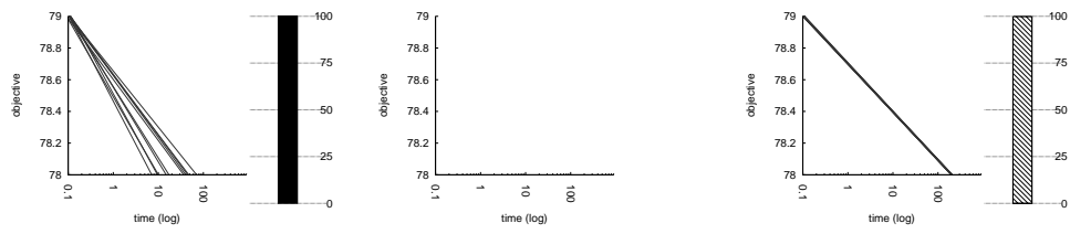
32.1 PGLNS
