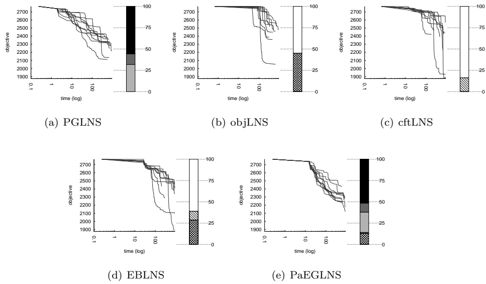
Fig. 10 Solving fastfood_ff58 instance with the five approaches.
