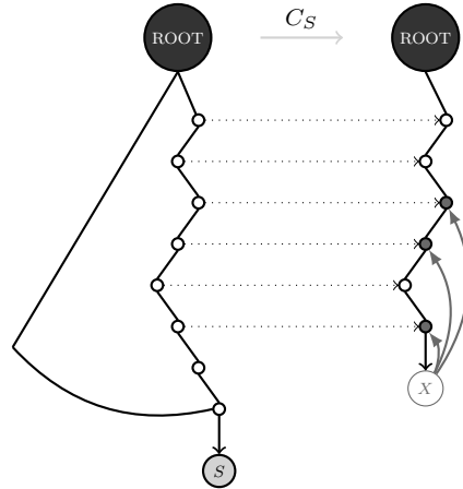
Fig. 1 Illustration of exp-cft .
