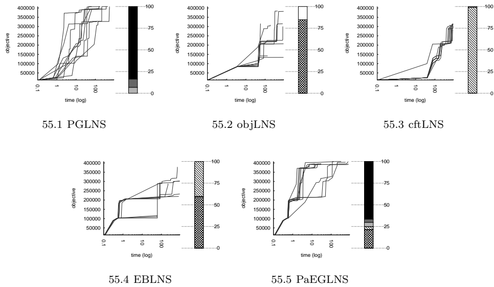
Fig. 55 ship-schedule.cp_7ShipsMixedUnconst.
