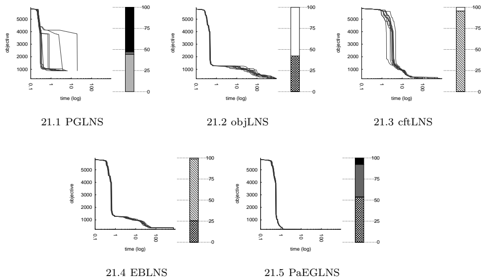
Fig. 21 fastfood_ff61.
