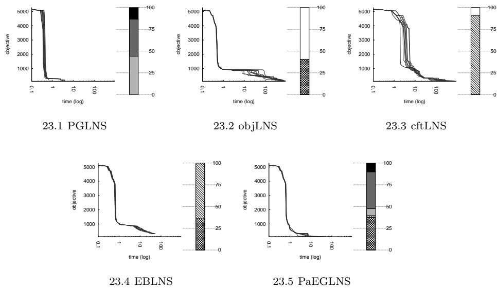
Fig. 23 league_model20-3-5.
