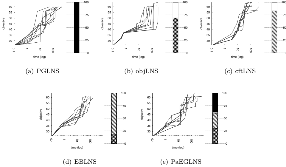
Fig. 11 Solving pc_30-5-6-7 instance with the five approaches.
