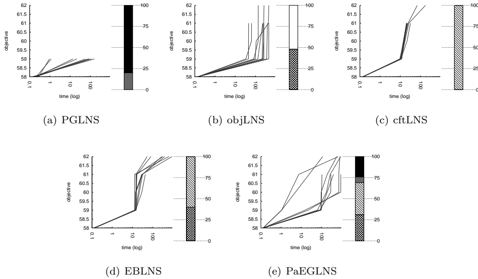
Fig. 12 Solving still-life_11 instance with the five approaches.
