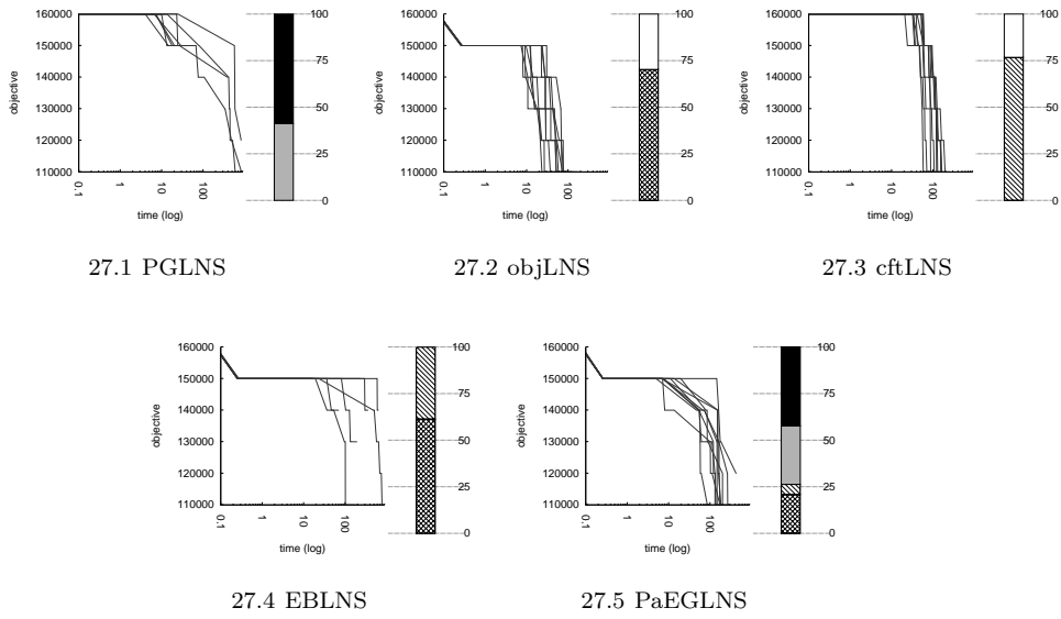
Fig. 27 league_model190-18-20.
