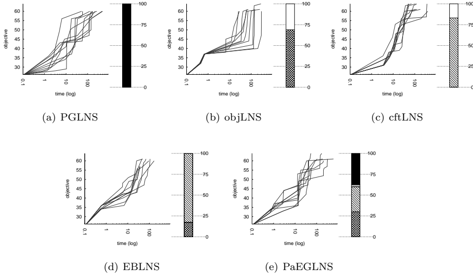
Fig. 11 Solving pc_30-5-6-7 instance with the five approaches.
