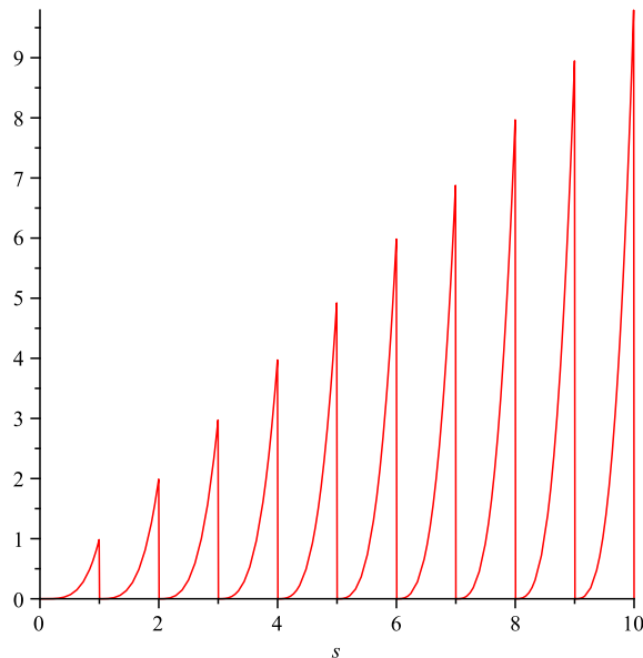
FIGURE 3. The function s \mapsto \{s\}^3 s
