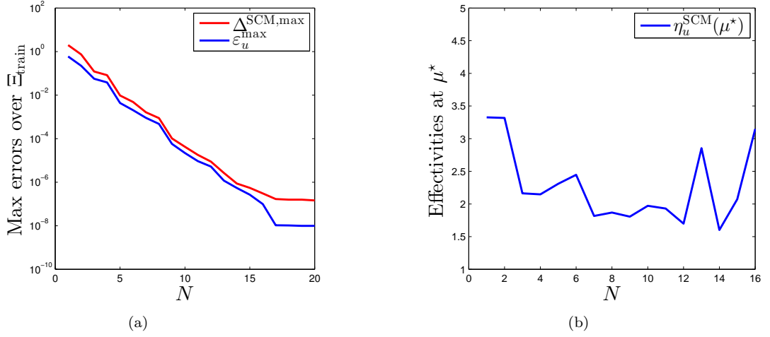
Figure 6: (a) Maximum of SCM upper error bound \Delta^{\text{SCM,max}} and displacement RB error \varepsilon_u^{\text{max}} over \Xi_{\text{train}} , and (b) displacement effectivity at \mu^* as functions of N (only first 16 iterations are shown in fig. 6(b)).
