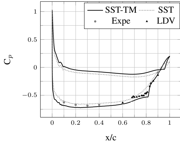
Figure 13: SST-TM and SST pressure coefficient distribution compared to experimental C_p from [6] (Expe) and [21] (LDV), AoA = 2^\circ , Re = 7.5 \times 10^5
