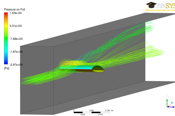
Figure 10: Streamlines of the 3D flow at \text{AoA} = 5^\circ \text{Re}=7.5 \times 10^5
