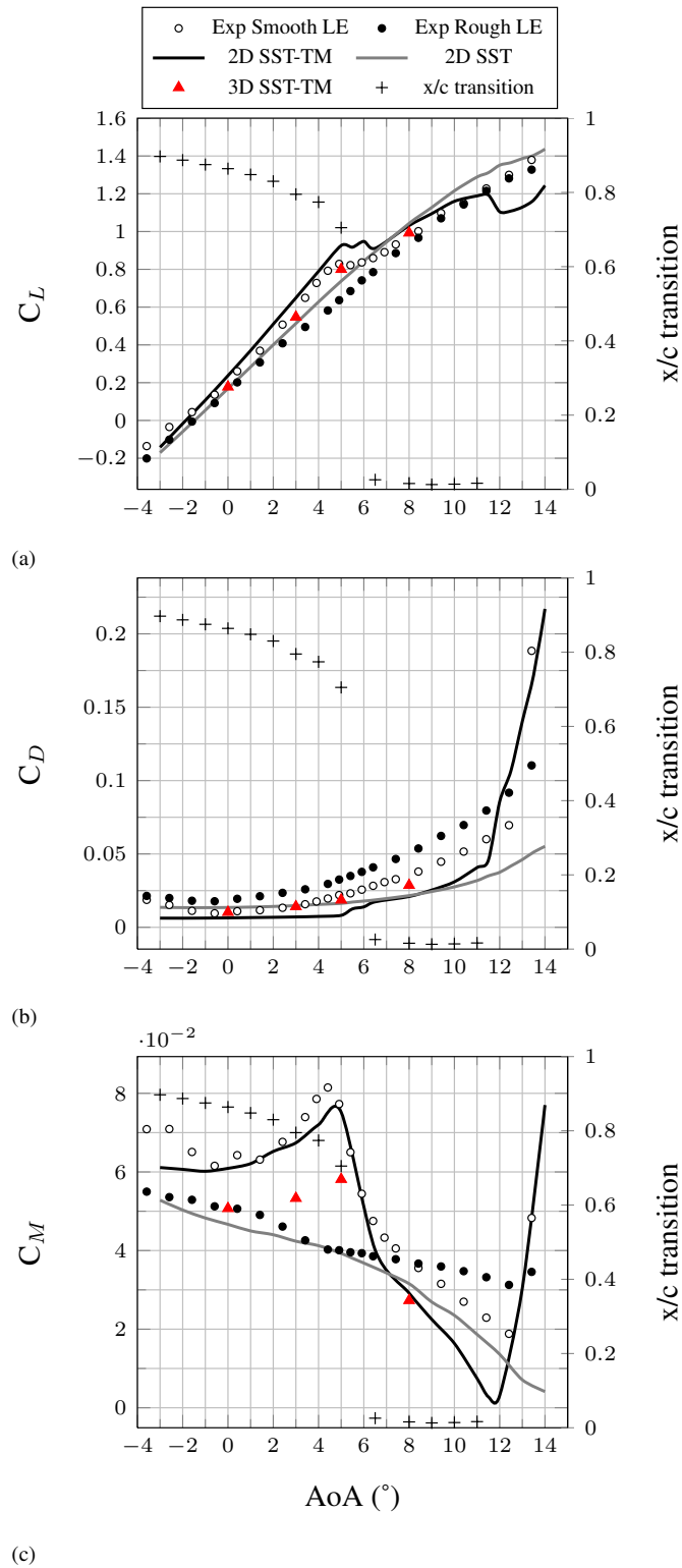
Figure 7: Experimental vs. numerical lift (a), drag (b) and moment (c) coefficients, Re = 7.5 \times 10^5 (the reader is referred to the web version of this article for an easier understanding of this figure: 3D marks are red triangles).
