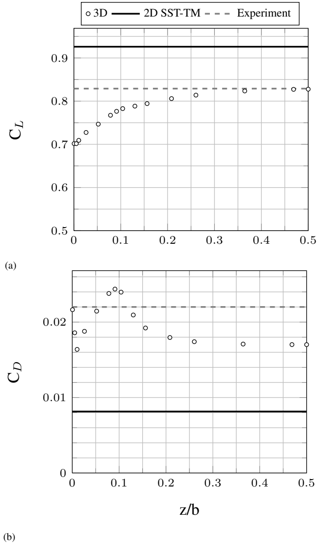
Figure 11: Spanwise distribution of lift (a) and drag (b) coefficients from the 3D calculation plus 2D SST-TM and experimental target values, AoA = 5^\circ , Re = 7.5 \times 10^5 . b = 0.192 m (total span of the hydrofoil)
