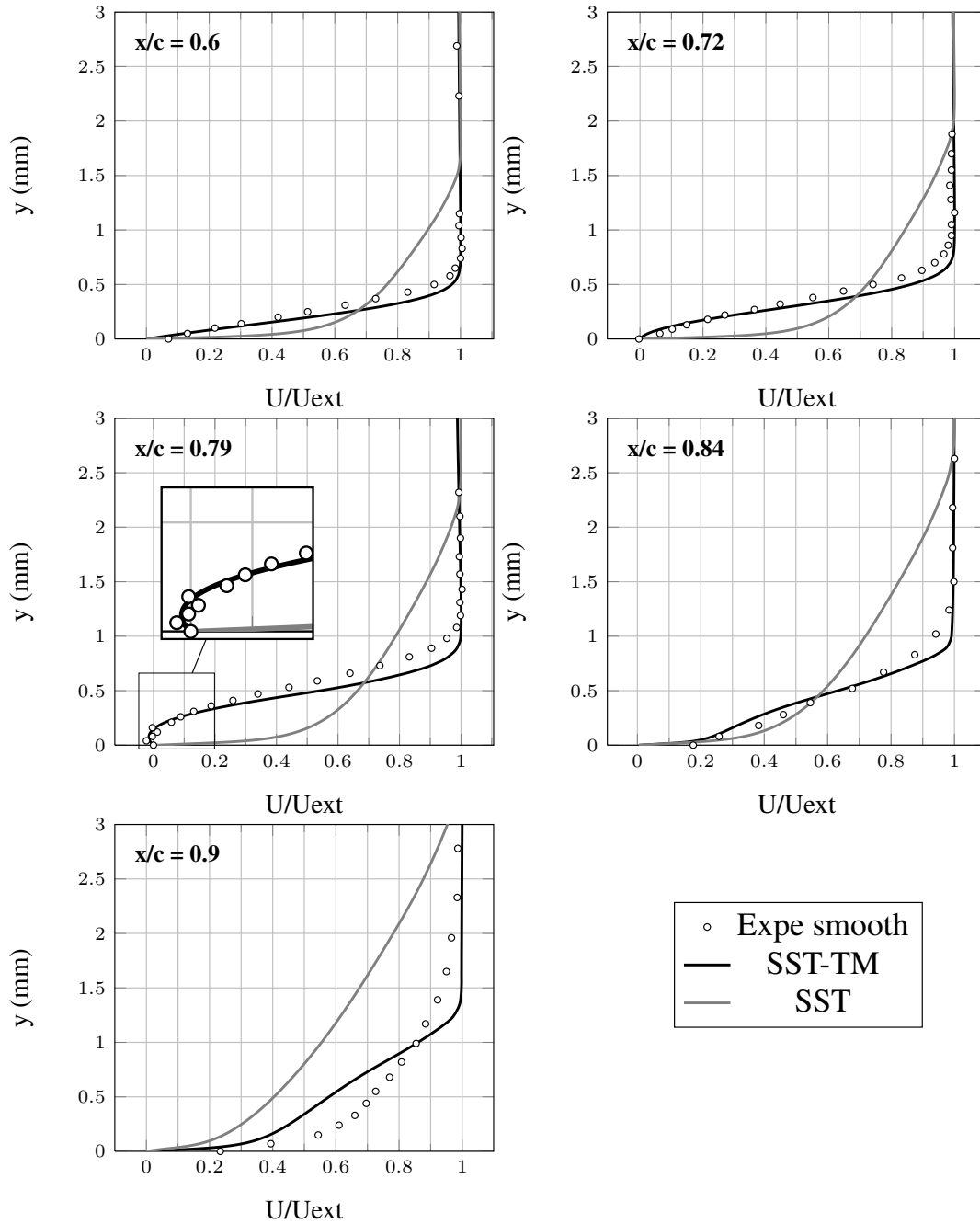
Figure 12: Velocity profiles in the vicinity of the LSB at 5 chord locations, \text{AoA} = 2^\circ , \text{Re} = 7.5 \times 10^5
