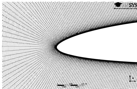
Figure 3: High-density mesh close to the leading edge
