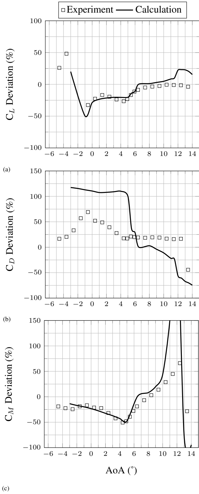
Figure 17: Deviations of experimental and numerical fully turbulent values of C_L (a), C_D (b) and C_M (c) relative to transitional values, Re = 7.5 \times 10^5
