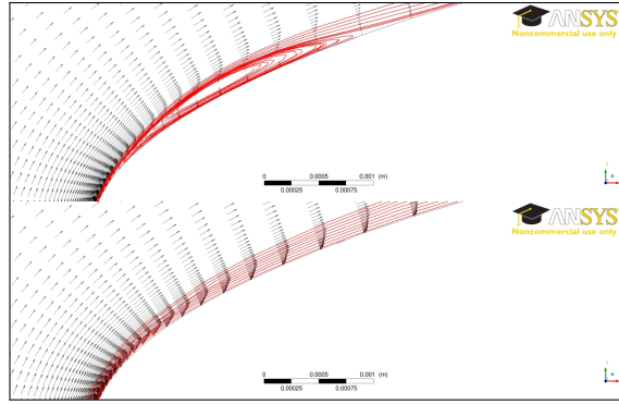
Figure 16: Velocity vectors and streamlines in the vicinity of the LSB for both SST-TM (top) and SST (bottom) models. \text{AoA} = 11^\circ , \text{Re} = 7.5 \times 10^5
