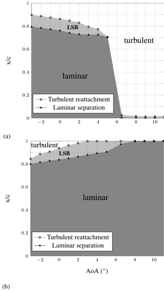
Figure 6: Laminar separation and turbulent reattachment locations on suction side (a) and pressure side (b) as a function of the angle of attack, Re = 7.5 \times 10^5
