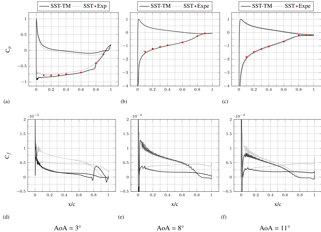
Figure 14: Pressure and friction coefficients at AoA = 3^\circ ((a) and (d)), 8^\circ ((b) and (e)) and 11^\circ ((c) and (f)), Re = 7.5 \times 10^5
