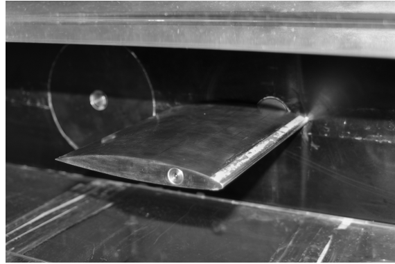
Figure 1: NACA 66(mod)-312 in the test section, with leading edge roughness
