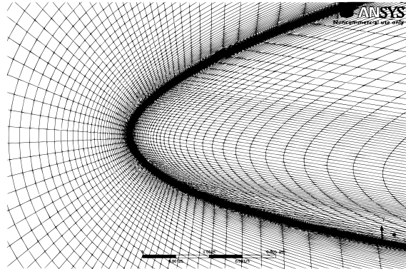
Figure 5: High-density mesh close to the leading edge and the side wall
