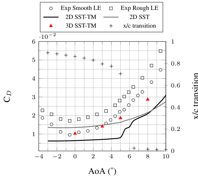
Figure 9: Experimental vs numerical drag coefficients, zoom of Figure 7 (b), Re=7.5 × 10 5 (the reader is referred to the web version of this article for an easier understanding of this figure: 3D marks are red triangles).
