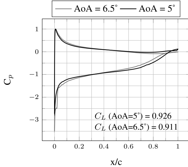
Figure 8: Pressure coefficient distribution at AoA = 5° and AoA = 6.5°, Re = 7.5 × 10 5
