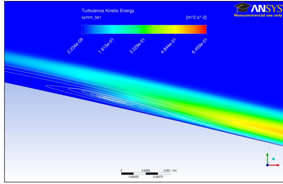
Figure 15: Turbulent kinetic energy contours and streamlines in the vicinity of the LSB ( x/c = 0.78 ).
