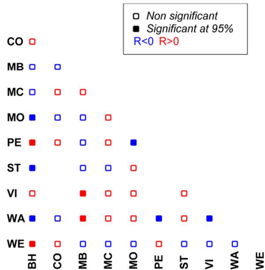
Figure 3. Correlation between the different SG time series as on Figure 2b, after removing a composite annual signal. The squared are filled when the correlation is significant (95% level). The coefficient is not evaluated when the time series overlapping is shorter than 3.5 years.
