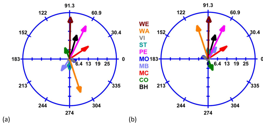
Figure 5. Phasor diagrams of the annual components obtained for the different SG time series before (a) and after (b) inverting the sign at the CO, MB, MO, ST, VI and WA underground stations. Amplitudes in \text{nm/s}^2 ; phases in days.
