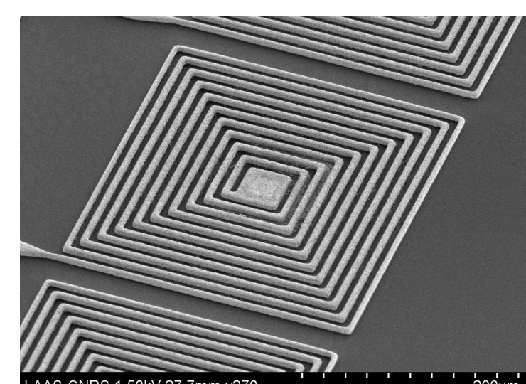
SEM picture of microfabricated spiral coil
