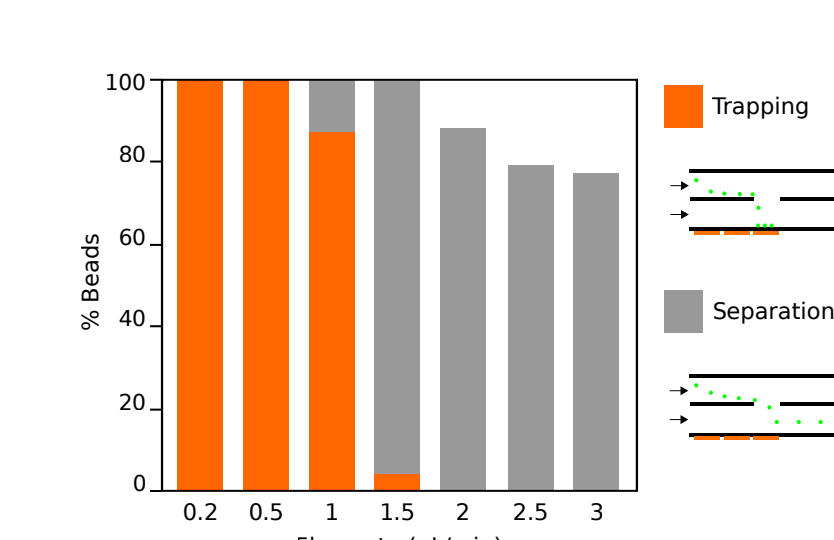
Impact of flow rate on beads trapping and separation efficiency
