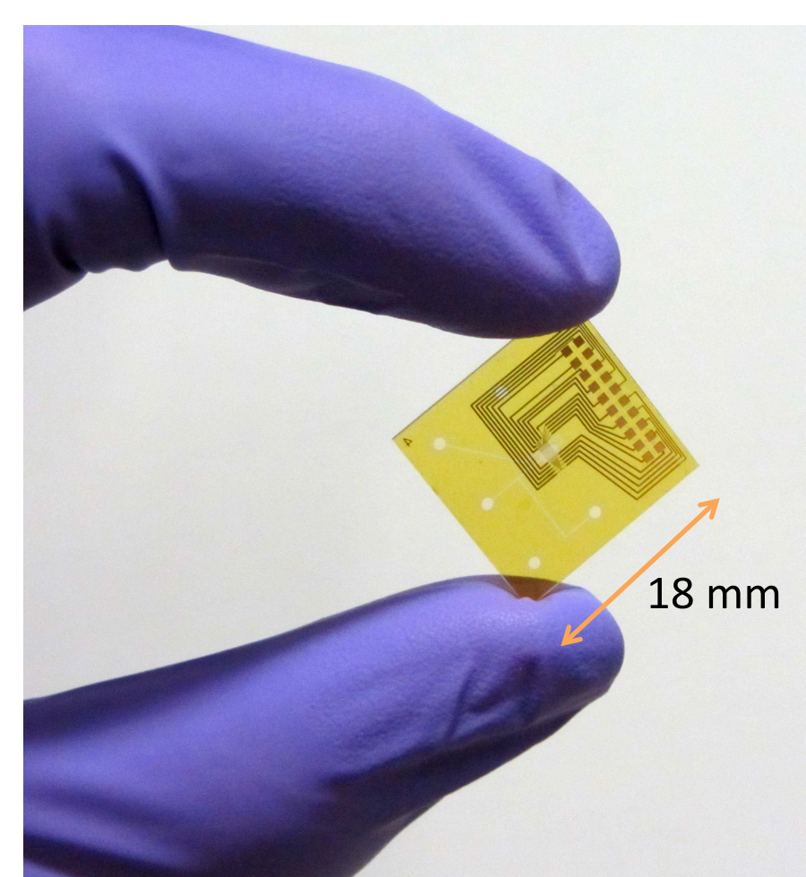
Microfluidic chip with 10 coils embedded
