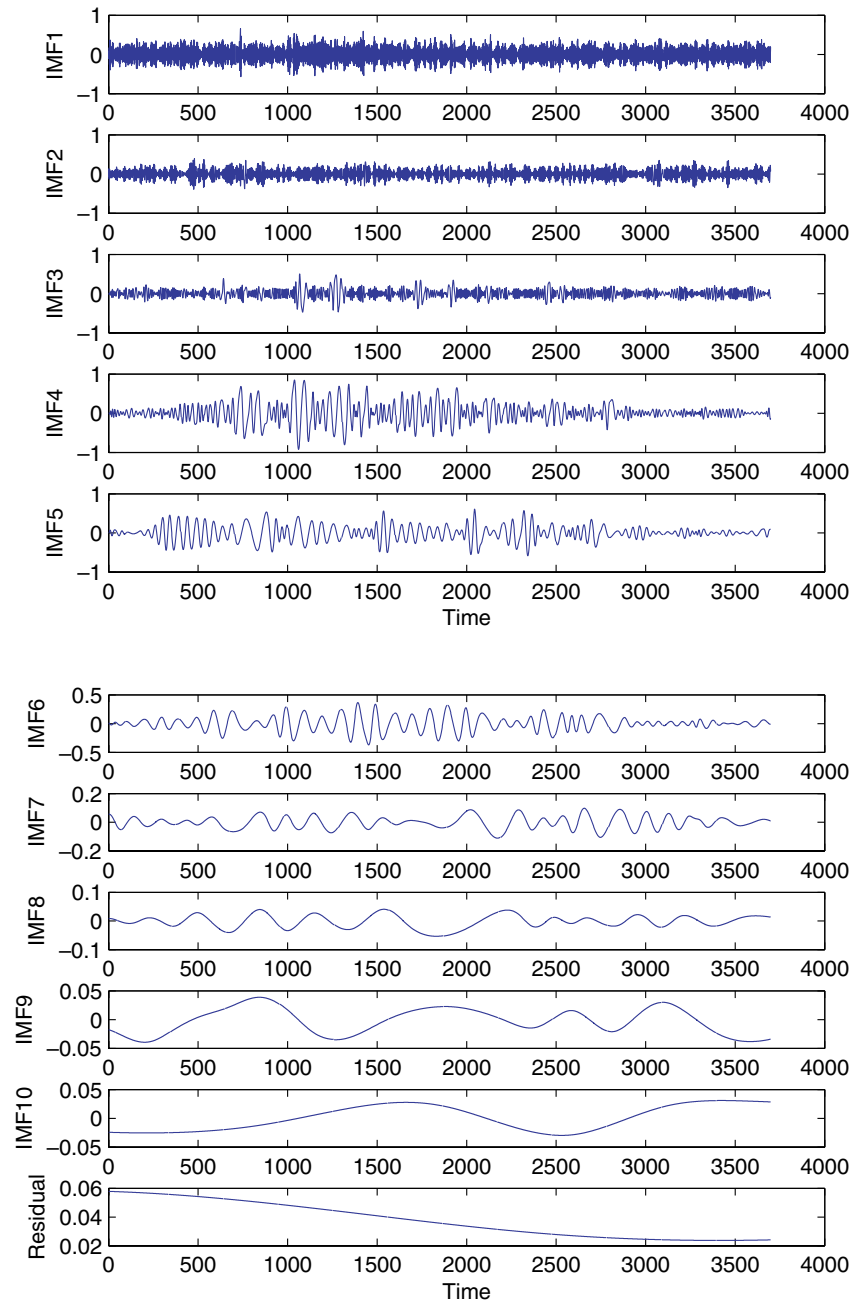
Fig. 5. Decomposition of noisy signal /o/ by EMD ( \text{SNR}_{\text{in}} = 2 \text{ dB} ).
