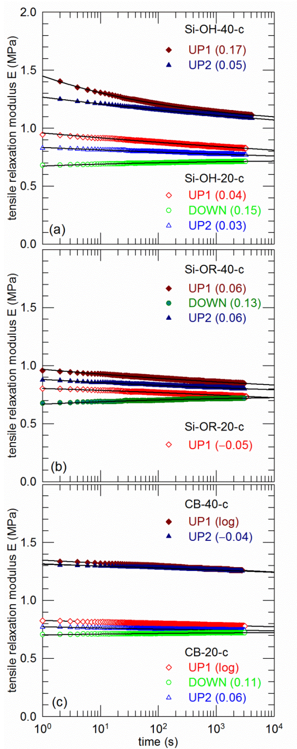
Figure 5. Time dependence of the tensile relaxation modulus E for \epsilon = 0.60 . The values of m are given in brackets.
