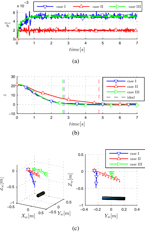
Fig. 9: Experimental results for the estimation of the radius of a cylinder with the following color coding: blue – case I, red – case II, green – case III. (a): behavior of \sigma_1^2(t) for the three cases (coincident for cases I and III and larger than in case II). (b): behavior of z(t) . The three vertical dashed lines indicate the times T_1 = 2.74 s, T_2 = 4.78 s and T_3 = 2.66 s at which the estimation error drops below the threshold of 2 mm. Note how T_1 \approx T_3 and T_1 < T_2 as expected. (c): two views of the camera trajectories for the three cases with arrows indicating the direction of the camera optical axis.
