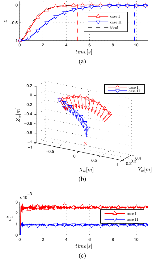
Fig. 6: Experimental results for the point feature case. (a): behavior of the estimation error for case I (solid red line) and case II (solid blue line), and for an ‘ideal’ second order system (9) with desired poles at \sigma_{max}^2 (dashed black line). The two vertical dashed lines indicate the times T_1 = 4.95 s and T_2 = 9.85 s at which the estimation error drops below the threshold of 5 mm. (b): Camera trajectories for case I (red line) and case II (blue line) with arrows indicating the direction of the camera optical axis. (c): behavior of \sigma_1^2(t) for case I (red line) and case II (blue line).
