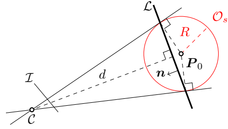
Fig. 2: Spherical target \mathcal{O}_s and planar limb surface \mathcal{L} .
