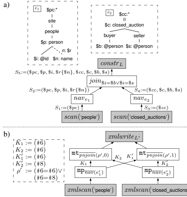
Fig. 13. Logical expression (a) and corresponding PACT plan (b) for the query in Example 4.
