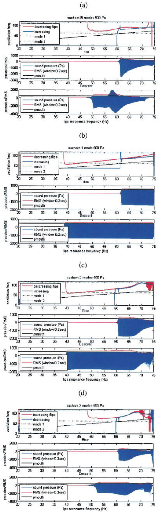
Figure 5: Saxhorn first regime simulations, p_{mouth} = 500Pa with respectively 15 (a), 1 (b), 2 (c) and 3 (d) mode(s) taken into account. Top plot : f_{osc} for rising (blue) and decreasing f_{lips} (red), first (black) and second (cyan) acoustic modes. Middle/top plots : radiated sound pressure and RMS envelope during f_{lips} rise/decrease.
