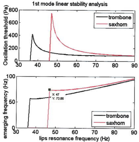
Figure 3: Results of Linear Stability analysis on first modes of the trombone (black) and the saxhorn (red). Top plot: the pressure thresholds of these modes (for different lips resonance frequencies). Bottom: the oscillation frequency at threshold.
