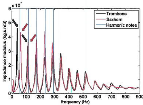
Figure 1: Module of the input impedance of a Saxhorn (red) and a Trombone (black). Blue vertical lines show the expected playing frequencies of first regimes. Arrows point the first and second modes of both instruments, the shift between first modes is easily noticeable.
