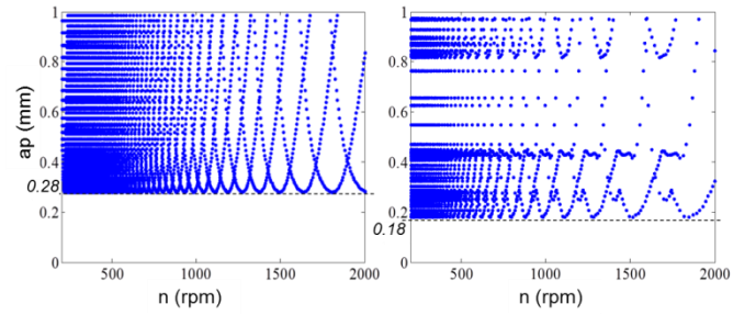
Fig. 12: Stability chart for the machining system : The spindle and the Tool_1 (on the left) and the spindle and the Tool_2 (on the right)
