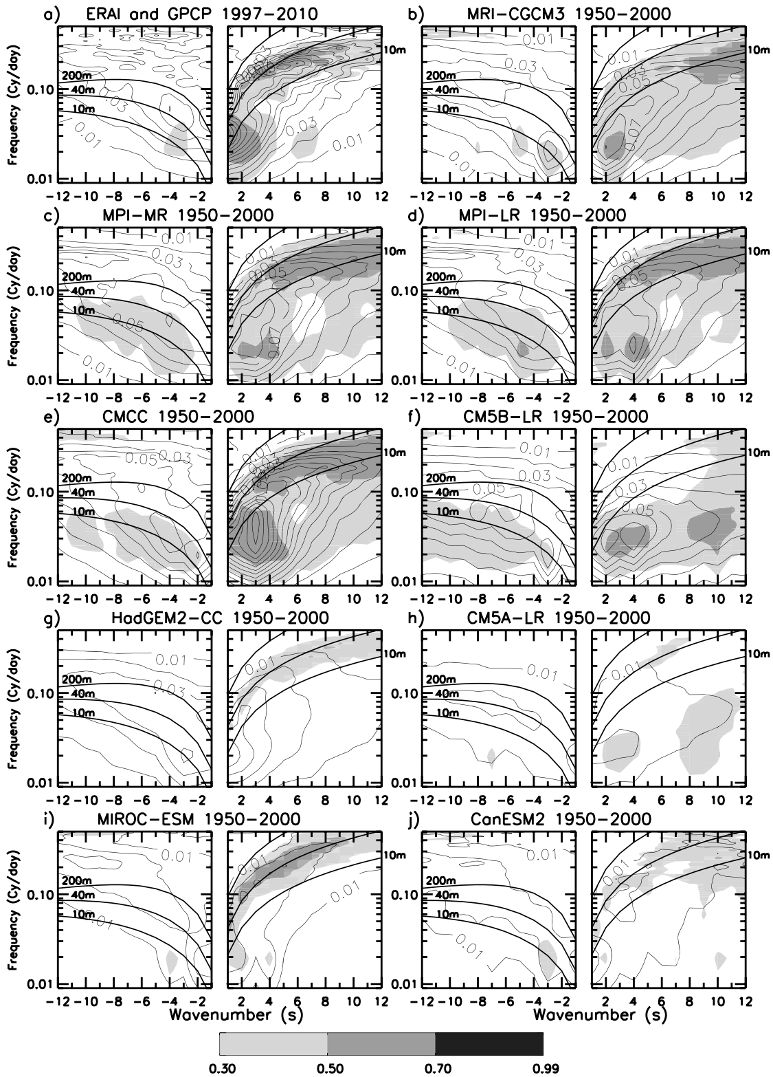
Figure 3. Spectra of symmetric precipitation (contour lines with interval= 0.01\text{ mm}^2\text{ day}^{-3} ) and of its squared coherency with the zonal wind at 850 hPa (shaded). The precipitation and wind are first tapered by a cosine function of 20^\circ width centered at the equator and averaged over ( 10^\circ\text{S} – 10^\circ\text{N} ) before their frequency-wave number periodograms are evaluated. The squared coherencies are then built from ratio between cross-spectra and spectra, those being estimated from averaged and smoothed yearly periodograms and cross periodograms exactly as described in Figure 1. All the coherency levels shown are above the 99% level (which is around 0.2 for r = 50 degrees of freedom). In all figures are also shown the dispersion curves for the n = 1 Rossby waves and Kelvin waves with equivalent depths h = 10, 40, 200\text{m} .
