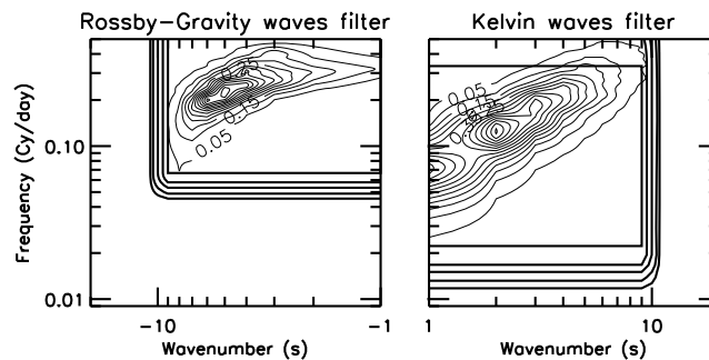
Figure 1. (left) Westward component of the 50 hPa spectra of the meridional wind (thin solid) and transfer function used to extract the Rossby-gravity waves (thick solid, contour interval=0.2). (right) Eastward component of the 50 hPa spectra of the zonal wind and transfer function used to extract the Kelvin waves. For all models the filters are identical but the spectra shown here are from ERAI data. To estimate the spectra, the fields are tapered in latitude by a cosine taper of 20^\circ width centered at the equator and then averaged in latitude over the equatorial band. Each year a time-longitude periodogram is then made and the spectra is estimated by averaging the periodograms over the years. The estimate of the spectra is further smoothed by applying 30 times a 1-2-1 filter in the temporal domain. This smooths the signal over around 15 points, yielding a spectral resolution of around 4 \cdot 10^{-2} cy/d.
