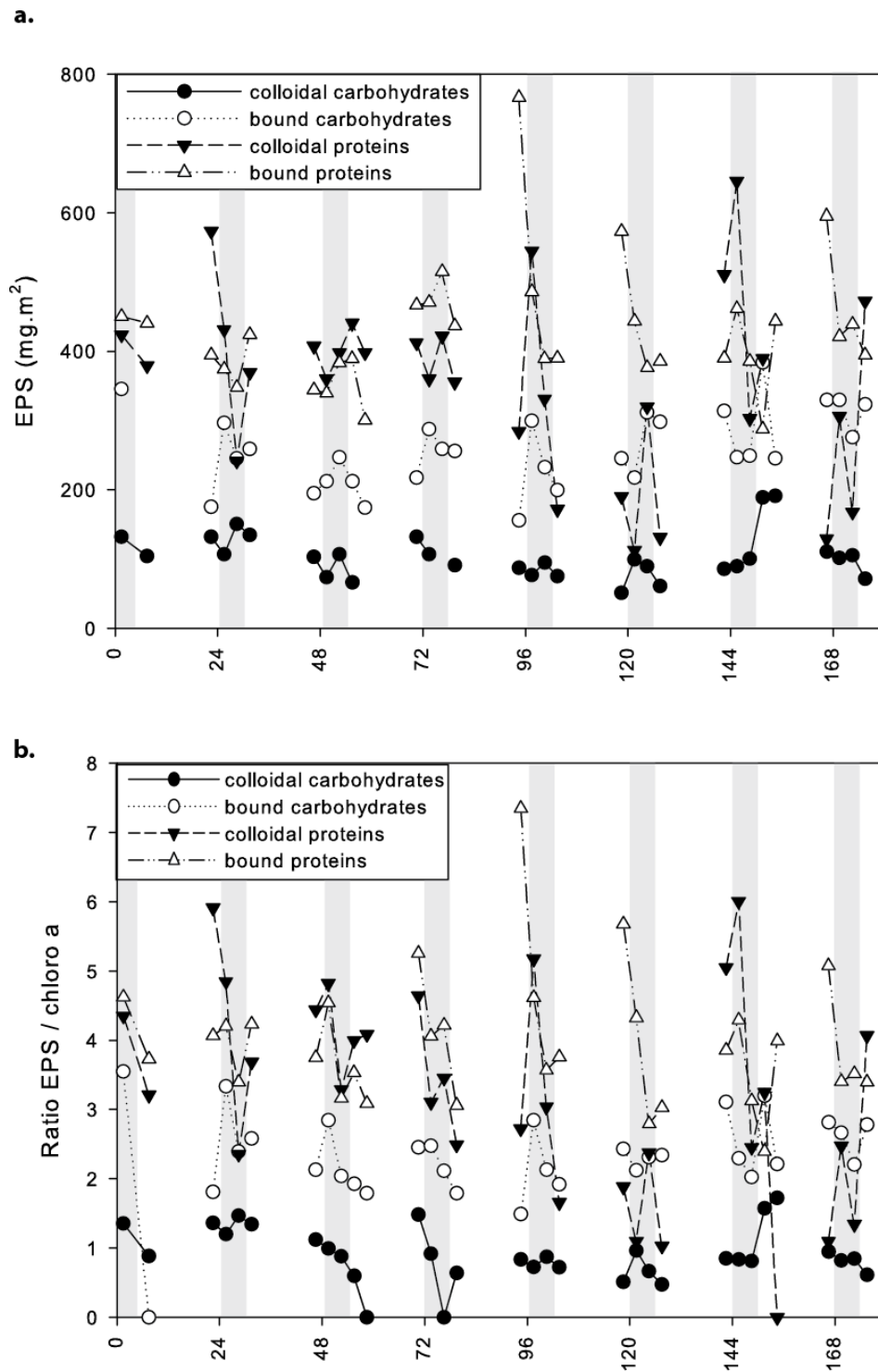
Figure 3 Figure 3: Temporal dynamics of a. the different fractions of EPS b. the ratio of different fractions of EPS to chlorophyll a concentrations. The gray bars indicate the low tides during the experiment.
