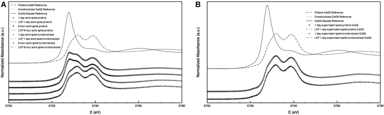
Figure 5. (A) XANES spectra obtained from the solids of a spike experiment with pristine and functionalized CeO 2 NPs and activated sludge where the particles and sludge were mixed for 8 h and 1 day and the Ce XANES spectra were subsequently probed. (B) XANES spectra from the supernatant spike experiment following 1 day of mixing with activated sludge.
