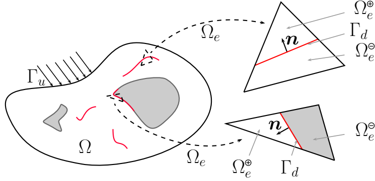
Figure 2: Illustration of the two kinds of discontinuous elements used in \Omega_e . On top right; a so-called matrix element embedded with only strong discontinuity and on bottom right; a interface element with both weak and strong discontinuity
