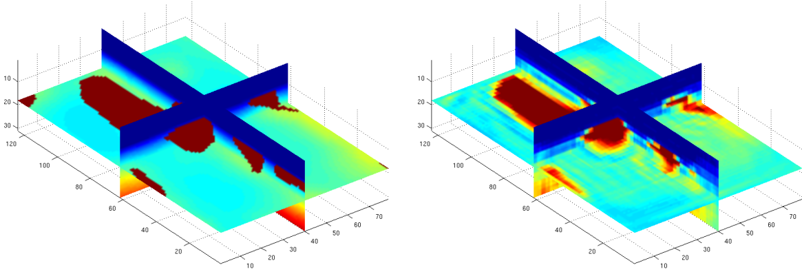
FIG. 11. The true wavespeed model (left) and the (partial) recovery at level 0 (right).
