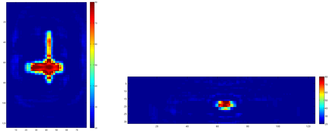
FIG. 28. Partial reconstruction of the quality factor at 15 Hz.
