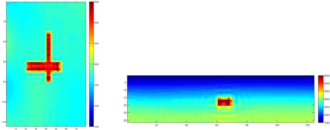
FIG. 27. Partial reconstruction of the phase velocity at 15 Hz.
