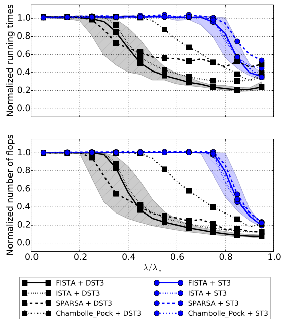
Figure 2: Normalized running times and normalized number of flops for solving the Lasso with a Pnoise dictionary.
