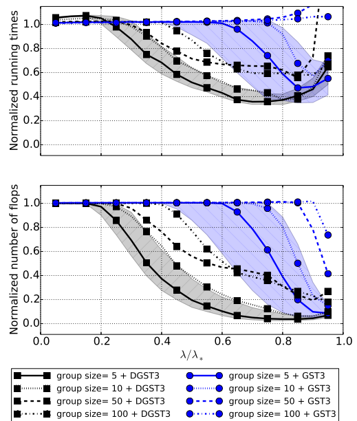
Figure 3: Normalized running times and number of flops for FISTA solving the Group-Lasso with different group sizes (5, 10, 50, 100).
