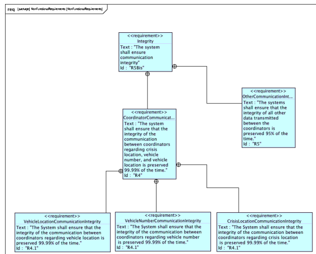
Fig. 4. Non-functional requirements in SysML
