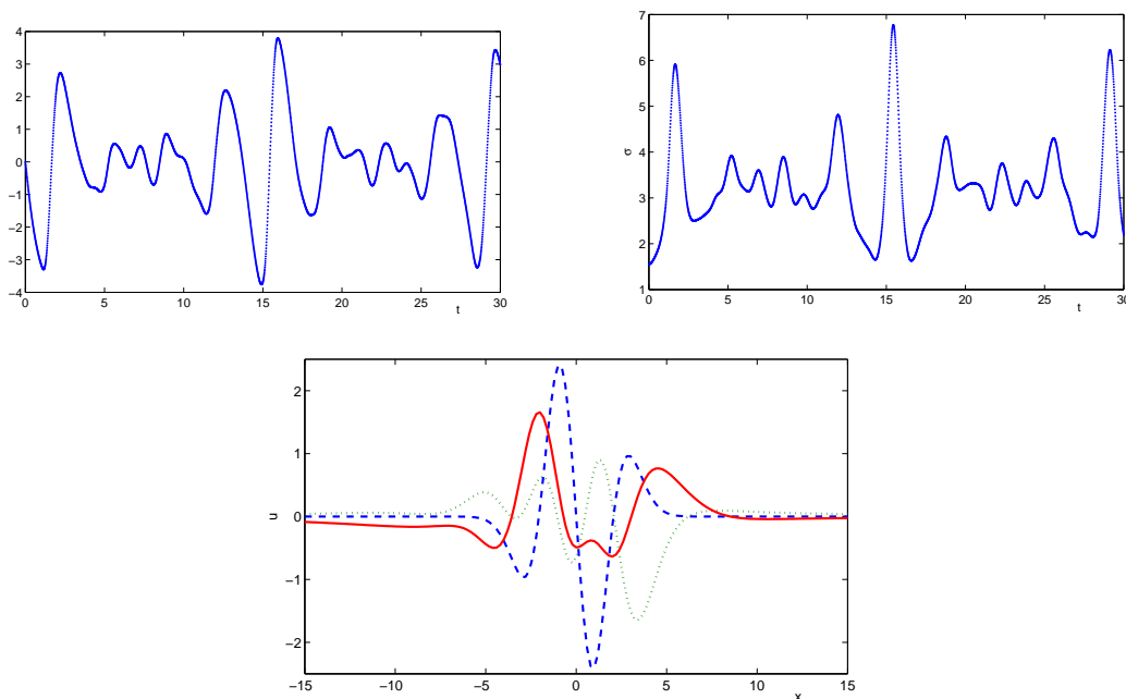
Figure 3: Numerical solution of the linearized log-KdV equation (1.7) with an odd initial data (4.9): center of mass \bar{x} (top left) and standard deviation \sigma (top right) versus time; the profile u(x, t) versus x (bottom) for t = 0 (blue dashed), t = 2.5 (green dotted), and t = 5 (red solid).
