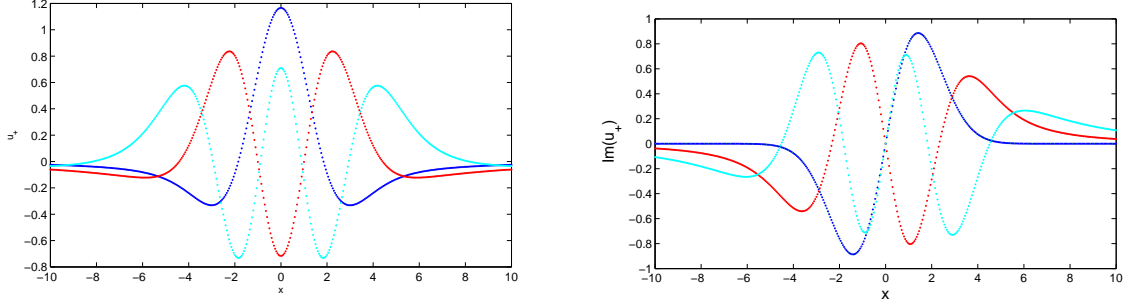
Figure 2: Real (left) and imaginary (right) parts of the three eigenfunctions u versus x for the first three eigenvalues E .
