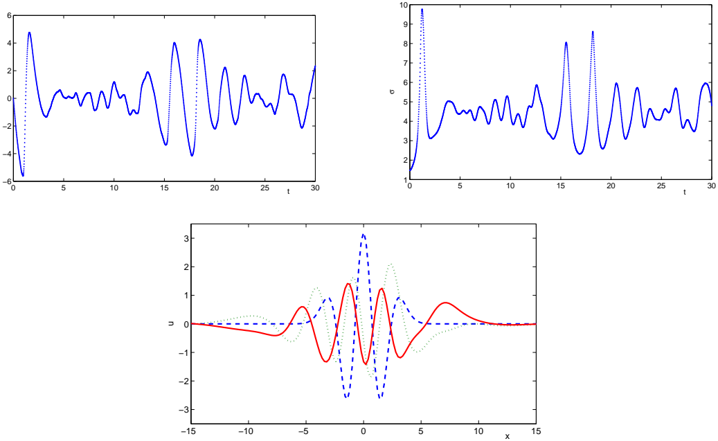
Figure 4: Numerical solution of the linearized log-KdV equation (1.7) with the even initial data (4.10): center of mass \bar{x} (top left) and standard deviation \sigma (top right) versus time; the profile u(x, t) versus x (bottom) for t = 0 (blue dashed), t = 2.5 (green dotted), and t = 5 (red solid).
