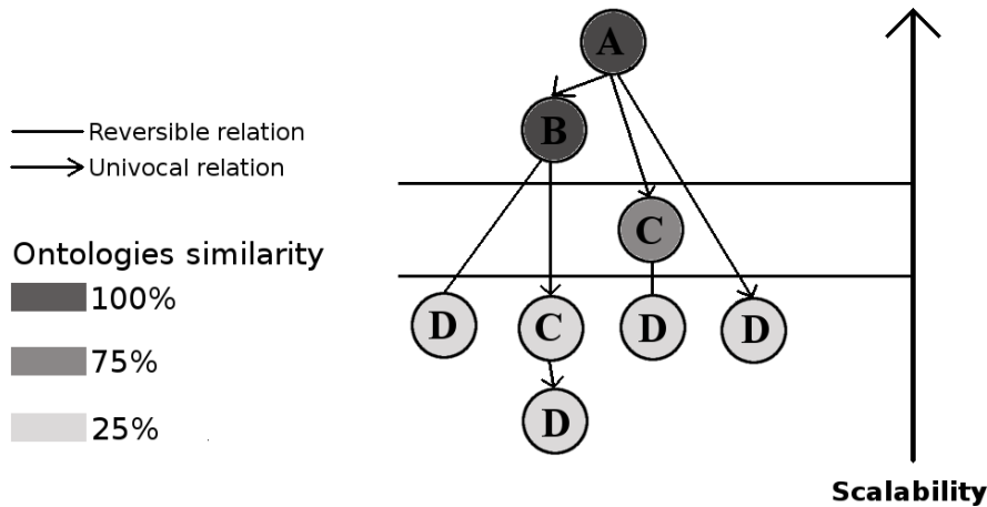
Figure 3. Ontologies classification.
