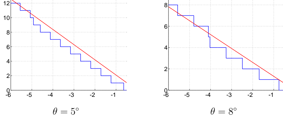
FIGURE 5. The blue line is the numerical computation of \mathcal{N}_{1-E}(\mathcal{H}_{\text{Gui}(\theta)}) as function of \ln_{10} E in abscissa. The red line is the asymptotics of Theorem 1.4. Mesh with 6416 triangles and #DOF = 120325.
