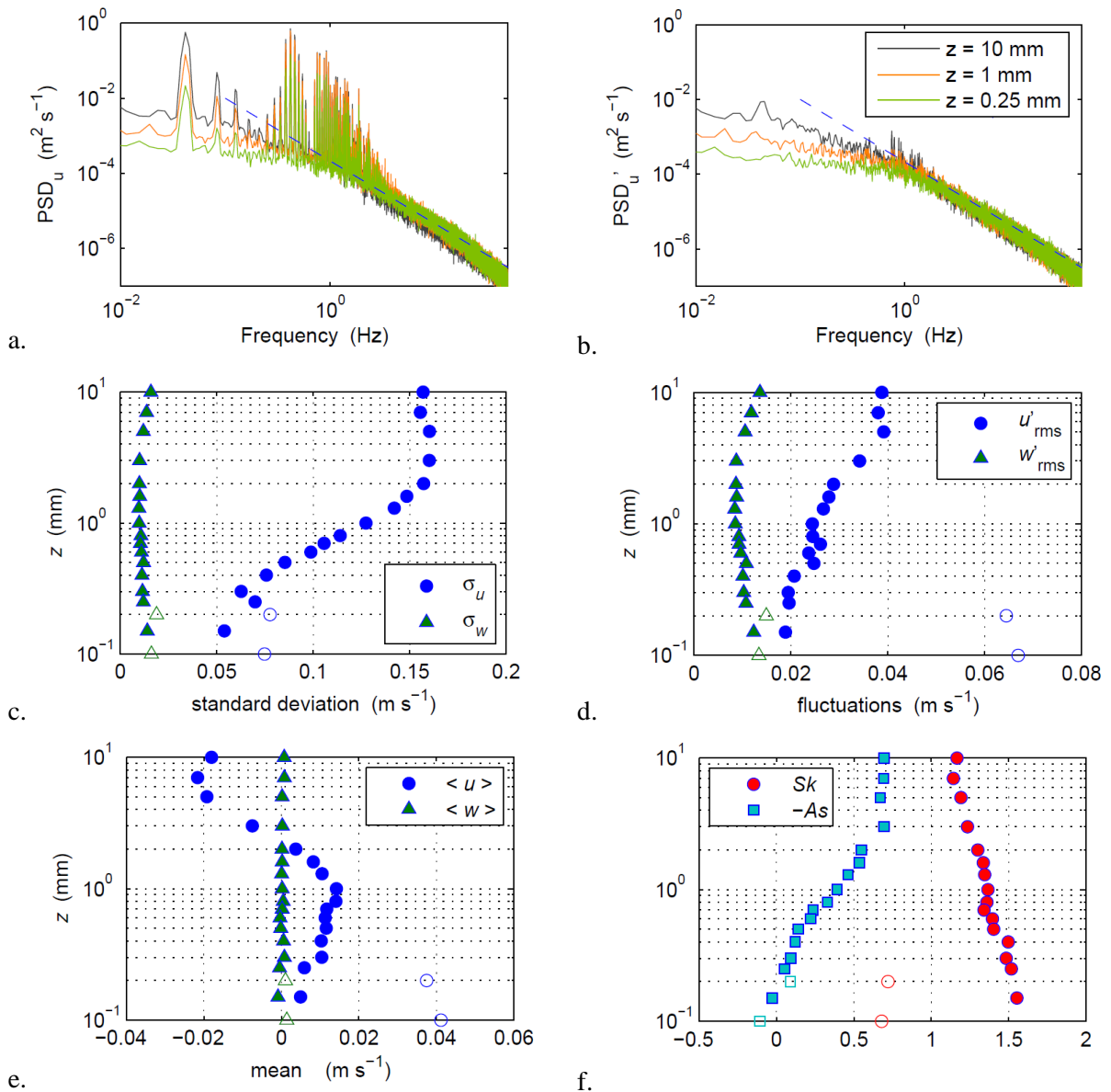
Figure 9. Example of boundary-layer measurements: (a) spectral density of horizontal velocities at three elevations above the bed and (b) with the ensemble average signal removed (the dashed line is the -5/3 slope); vertical profiles of: (c) standard deviation of horizontal and vertical velocities, (d) their fluctuations, (e) mean values; (f) skewness and asymmetry of u . The blank symbols stand for measurements made without seeding material.
