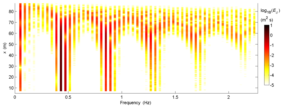
Figure 4. Logarithm of energy density E_d as a function of frequency f and cross-shore position x for condition B3. The energy is concentrated at the multiples of (f_2-f_1) for which the lines have been thickened into stripes for readability.
