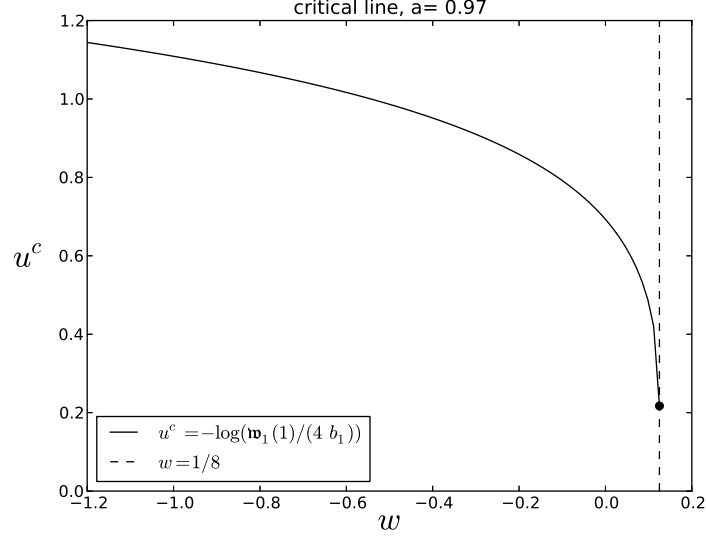
FIGURE 1. The critical line u^c = -\log\left(\frac{\mathfrak{w}_1(1)}{4b_1}\right) .
