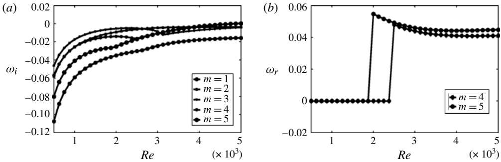
FIGURE 7. Plots as a function of the Reynolds number Re of the leading modes associated with different azimuthal wavenumbers m , in the setting where W = 0.5 and H = 0.5 : (a) temporal growth rates \omega_i ; (b) oscillation frequencies \omega_r .
