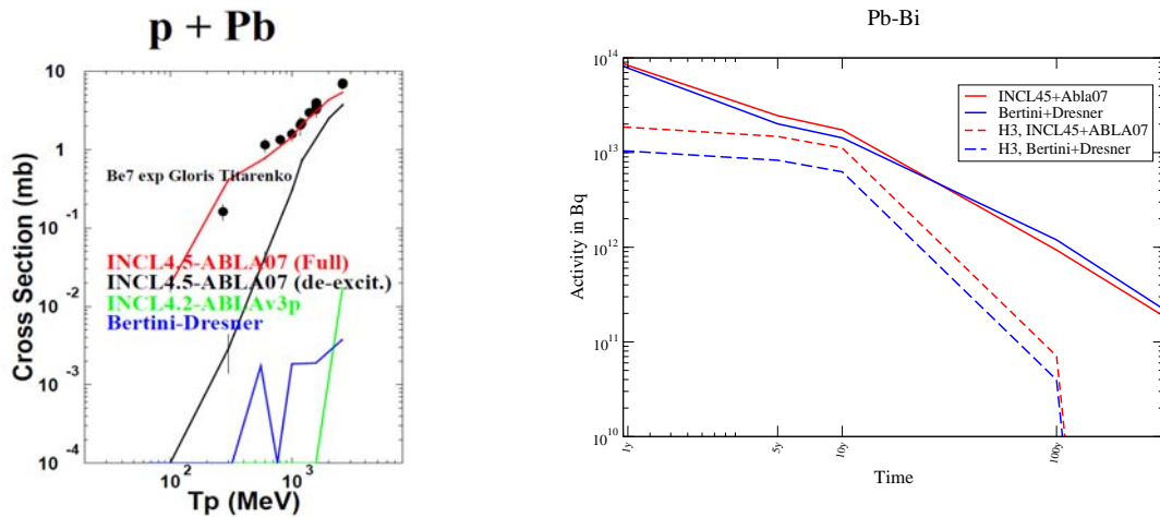
Figure 10.5.6: Left: 7 Be production cross-section in lead. Right: Total activity (solid lines) and activity due to tritium (dashed lines) in the liquid Pb-Bi of the MEGAPIE target calculated with MCNPX using the INCL4.5-ABLA07 (red lines) or the Bertini-Dresner (blue lines) models. From [10.5.18].
