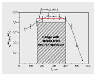
Figure 10.2.2 \bar{\sigma}_f(^{238}U) / \bar{\sigma}_f(^{235}U)
