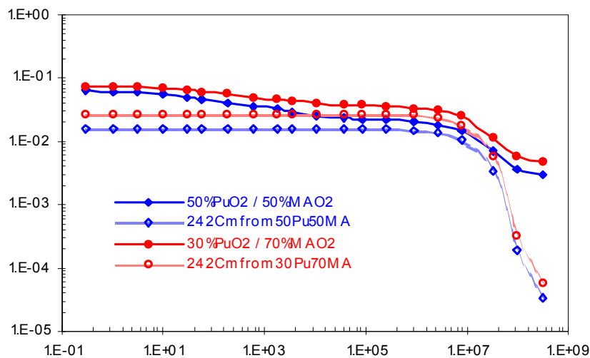
Figure 3.6: Normalized decay heat and ^{242}\text{Cm} contribution.
