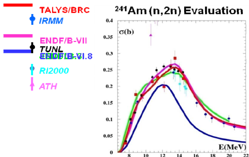
Figure 10.5.2: ^{241}\text{Am}(n,2n) Evaluation
