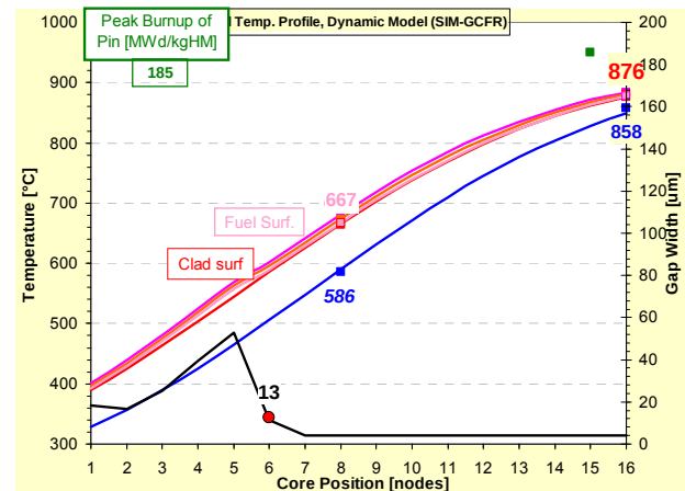
q) Axial peak pin temperature profile 2000 sec into PLOF at EOC
