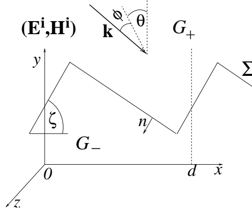
Figure 12.2: Cross section of a simple grating of period d with incidence direction \mathbf{k} , incidence angle \theta and conical angle \phi .
