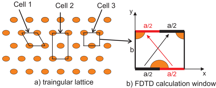
Figure 9.7: Triangular structure and FDTD calculation window
