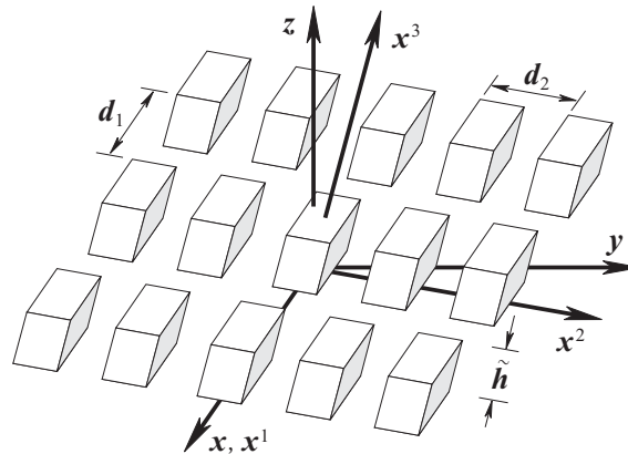
Fig. 13.6. Definition and notation of a crossed grating problem. All surfaces of the rhombs are parallel to a coordinate surface of the skew Cartesian coordinate system Ox^1x^2x^3 defined in Fig. 13.7.
