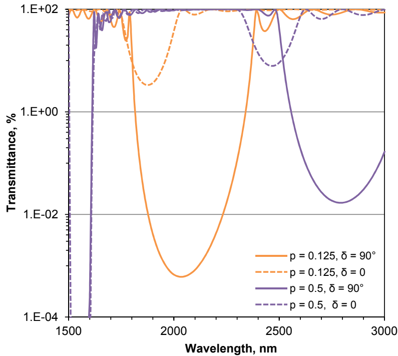
Figure 12.20: Calculated transmission spectra of 1 \mu\text{m} -period gratings with 15 layers of dielectric circular rods with \epsilon = 4 and different filling ratios p embedded in vacuum with hexagonal structure, plotted vs. \lambda for \theta = 0 , \phi = 0 and different polarization angles (classical diffraction).
