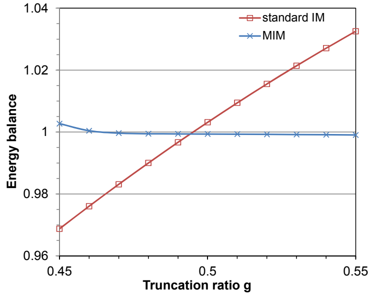
Figure 12.16: Energy balance vs. g used for the same diffraction problem as in Fig. 12.15, but for N = 400 .
