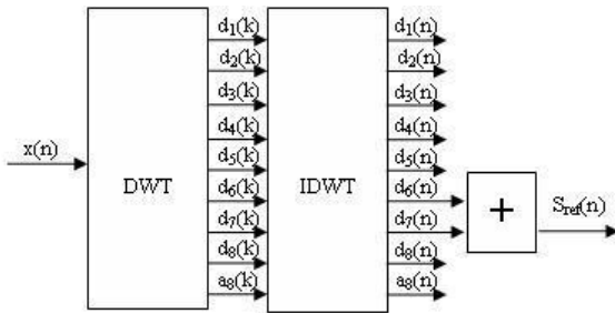
Figure 1: Reference signal extraction: The contaminated ECG is decomposed into 8 scales using the discrete wavelet transform. The details are then reconstructed and a reference signal is formed by summing details 6 and 7, hence covering the 4-16 Hz sub-band.
