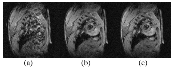
Figure 5: Mouse cardiac MRIs acquired with a GE sequence: (a) with no synchronization, (b) with cardiac gating, (c) with cardio-respiratory gating.
