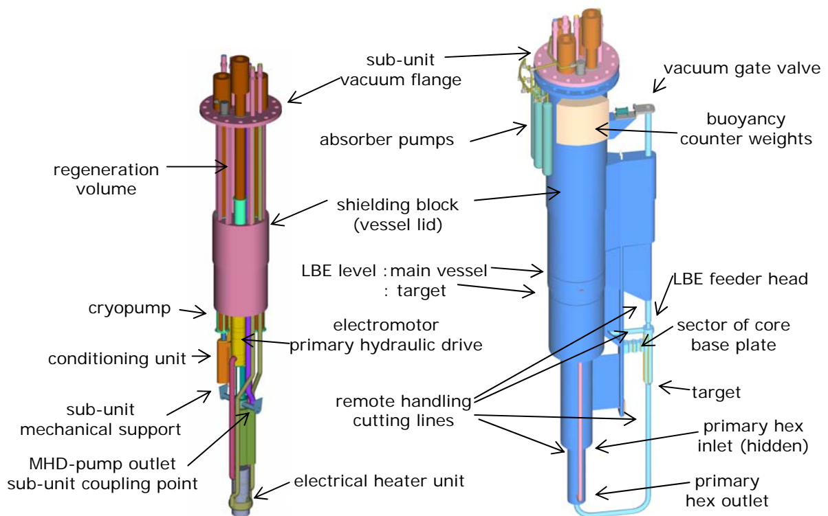
Figure 2. Spallation sub-unit and outside housing of the spallation loop (Draft-2)
