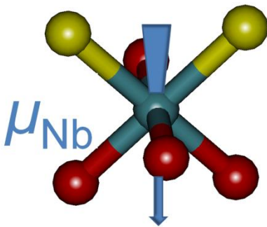
Figure 3. Orthorhombic 4 short (red, R_1 = 1.94 (1) \text{ Å} ) – 2 long (yellow, R_2 = 2.15 (1) \text{ Å} ) distribution of Nb-O bond distances along with \langle 110 \rangle Nb-off center \mu_{\text{Nb}} .
