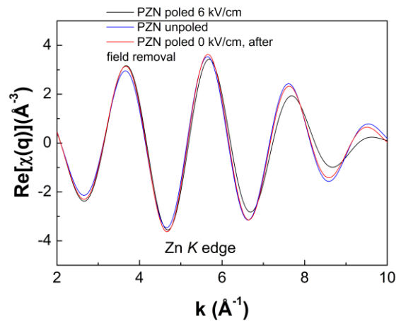
Figure 6. Backward Fourier transform in the k^3 -weighted space calculation obtained for an unpoled sample (blue), a sample poled at 6 kV/cm (black) and a poled sample (red) after removal of the electric field (0 kV/cm).
